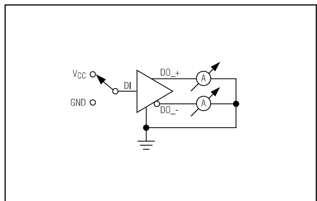
Figure 6. Short-Circuit Measurements
