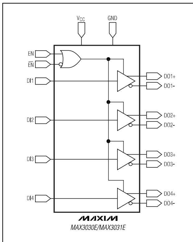
Figure 15. MAX3030E/MAX3031E Functional Diagram
