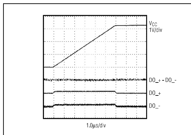
Figure 13. Differential Power-Up Glitch (1V/μs)
