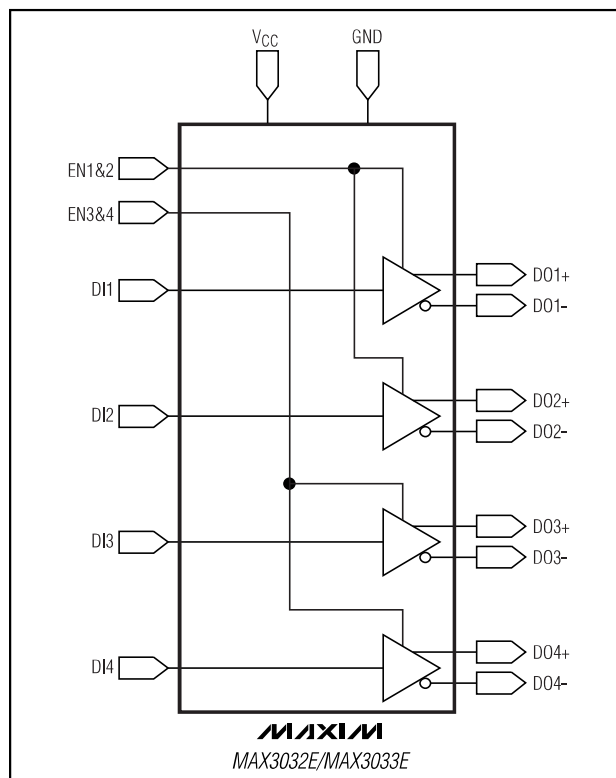
Figure 16. MAX3032E/MAX3033E Functional Diagram
