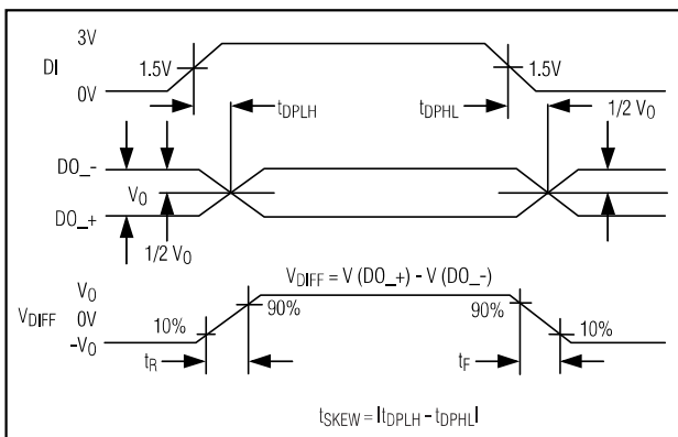
Figure 3. Differential Driver Propagation Delay and Transition Waveform
