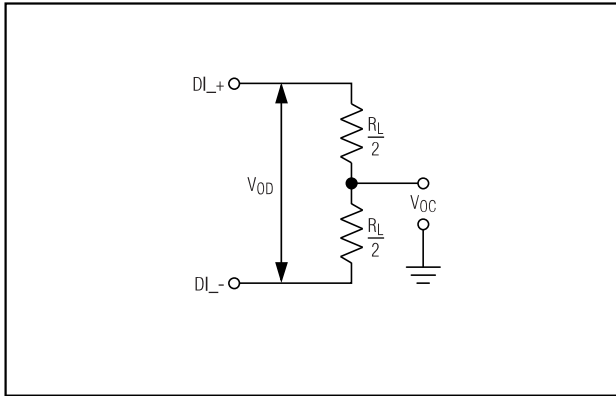
Figure 1. Differential Driver DC Test Circuit
