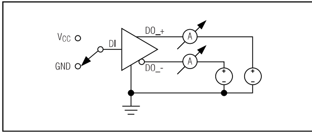
Figure 7. Power-Off Measurements
