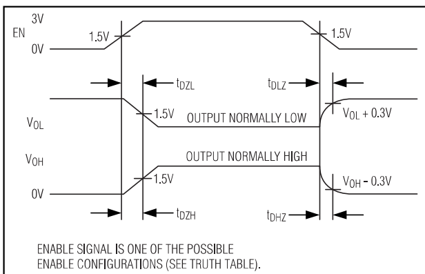
Figure 5. Driver Enable/Disable Waveform
