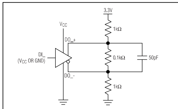
Figure 11. Differential Power-Up Glitch (Hot Swap)
