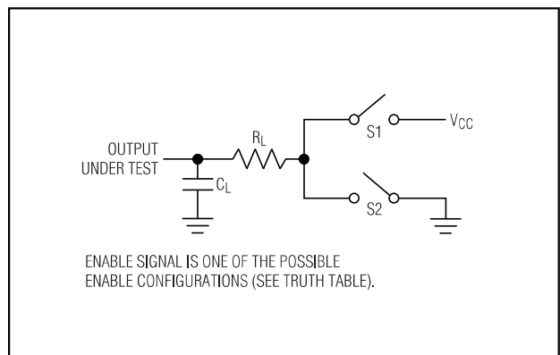
Figure 4. Driver Enable/Disable Delays Test Circuit
