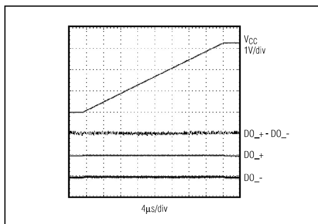
Figure 12. Differential Power-Up Glitch (0.1V/μs)
