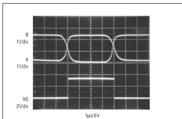
Figure 18. MAX3483/MAX3488 Receiver Propagation Delay
