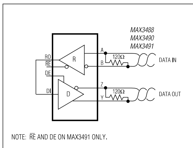
Figure 23. Line Repeater for MAX3488/MAX3490/MAX3491
